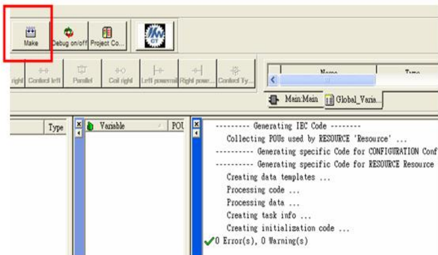
Fig. 5 Editing Screen
